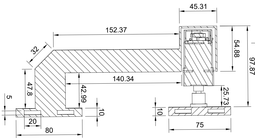
Section View A-A (1:1.75)
