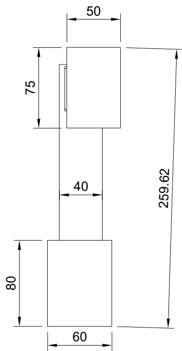
View B Bottom view (1:25)
