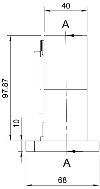
View A Side View (1:1.5)
